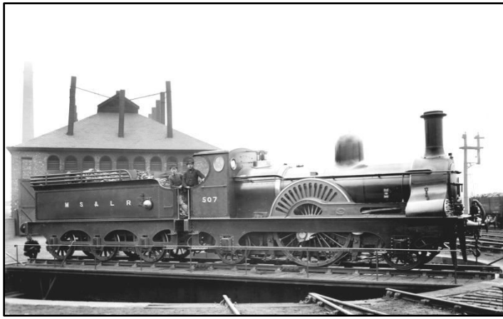
MS&LR class 14 2-2-2 no.507
